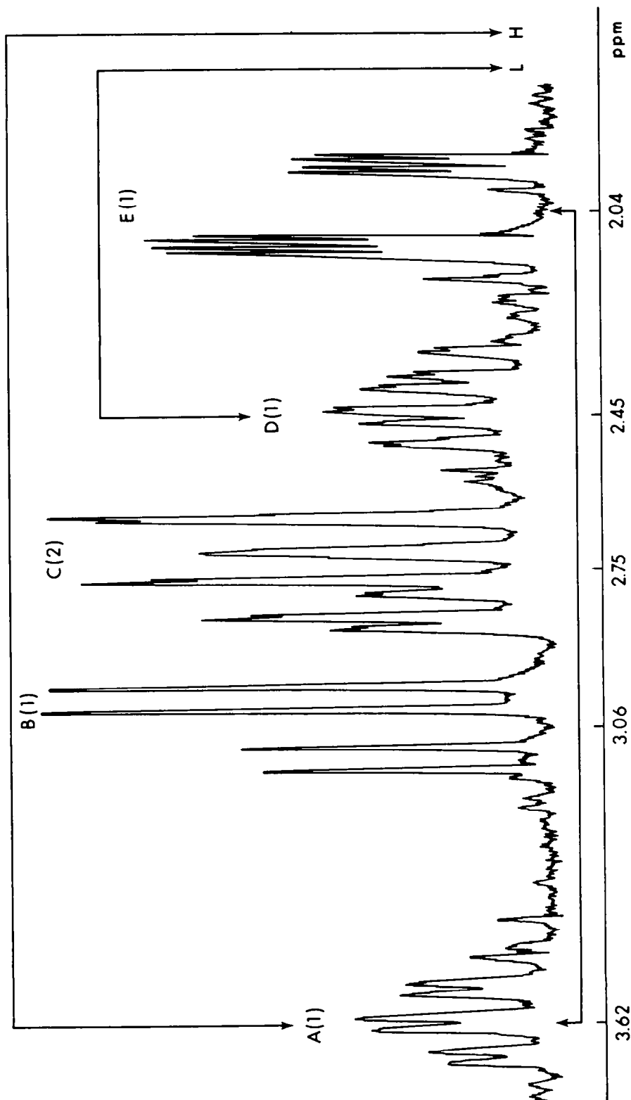
Part of the 100 MHz spectrum of 1- t -butyl-2,5-dimethyl-4-piperidone in \text{CDCl}_3 , sweep width 250 Hz. L and H denote the lower and higher s -methyl doublets respectively. The integral of each group is given in parenthesis after its letter of identification. Arrows indicate some of the spin systems established by decoupling experiments.
